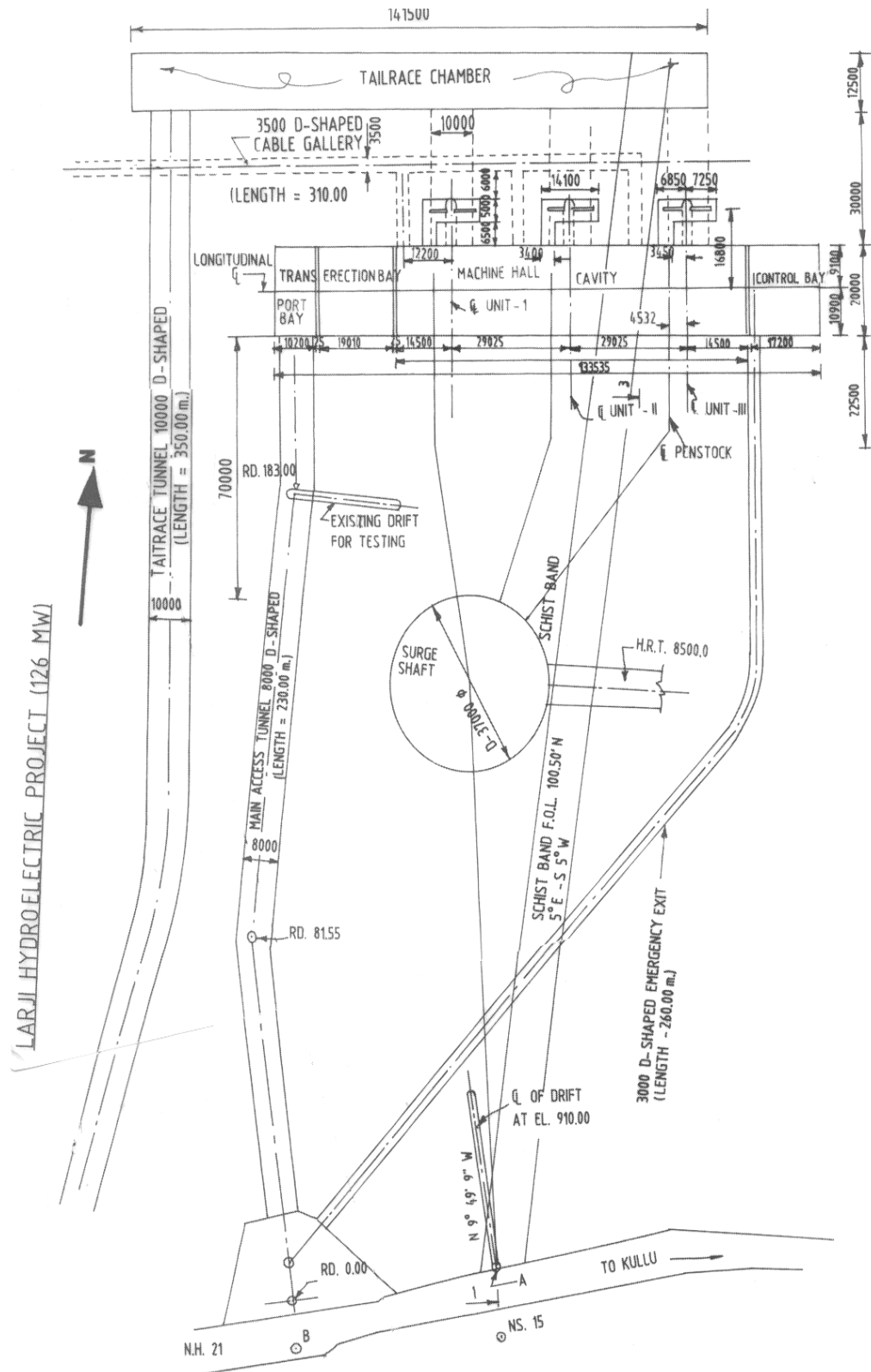
Fig. 2 - Plan of underground powerhouse and the testing drift
