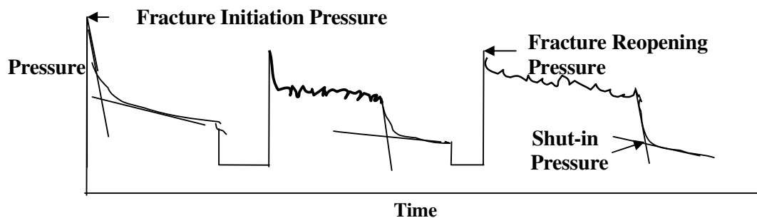
Fig. 5 - Pressure time record of hydraulic fracturing test
