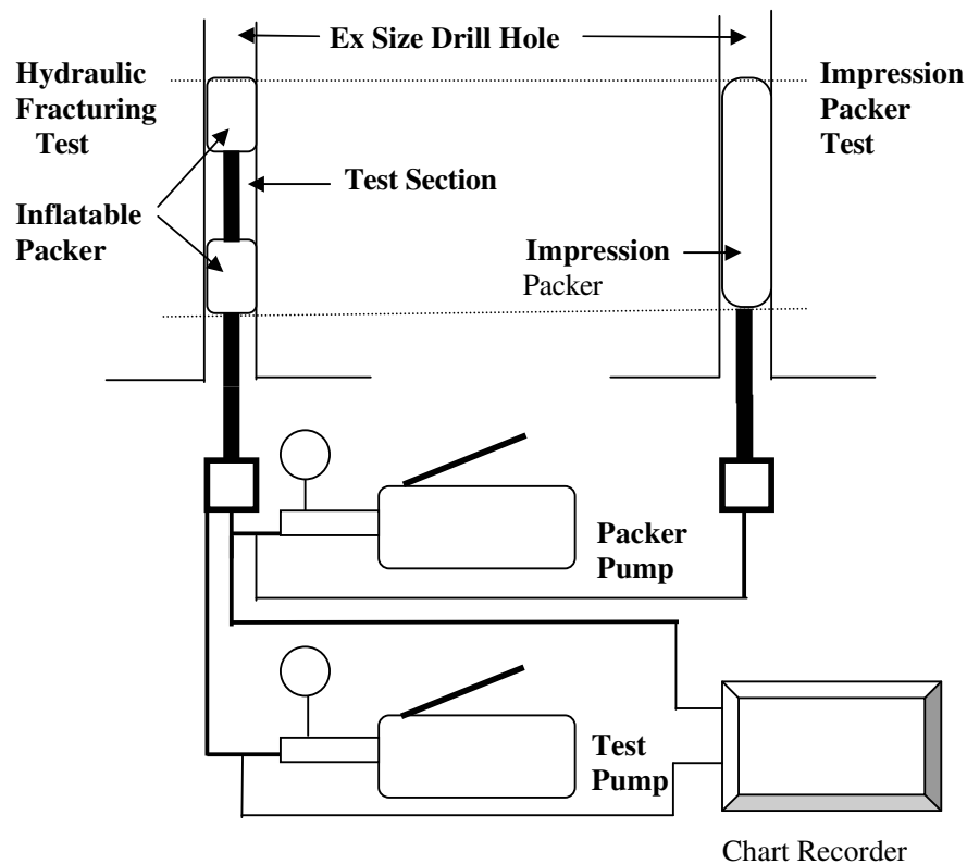
Fig. 3 - Schematic diagram of hydraulic fracturing equipment
