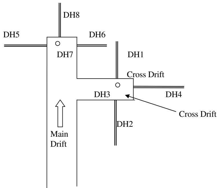
Fig. 6 - Locations of the drill holes in powerhouse at RD 188m + 34 m (cross drift) and at RD 197 m (main drift)
