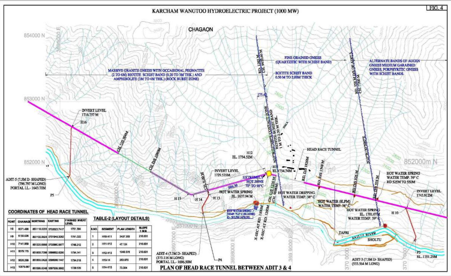
Fig. 4 - Plan of HRT between adits 3 and 4
