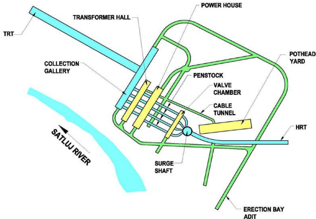
Fig.1 - Layout of works at powerhouse site
