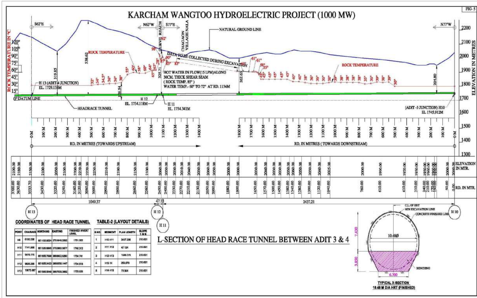
Fig. 5 - L-section of HRT between adits 3 & 4 showing rock temperature
