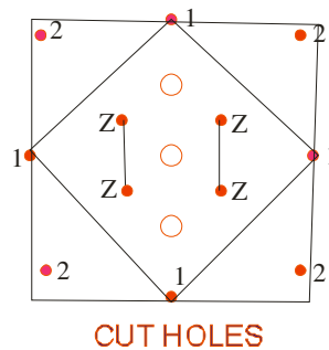
Fig. 7 – Drilling and blasting pattern for Adit 4 (upstream) HRT
