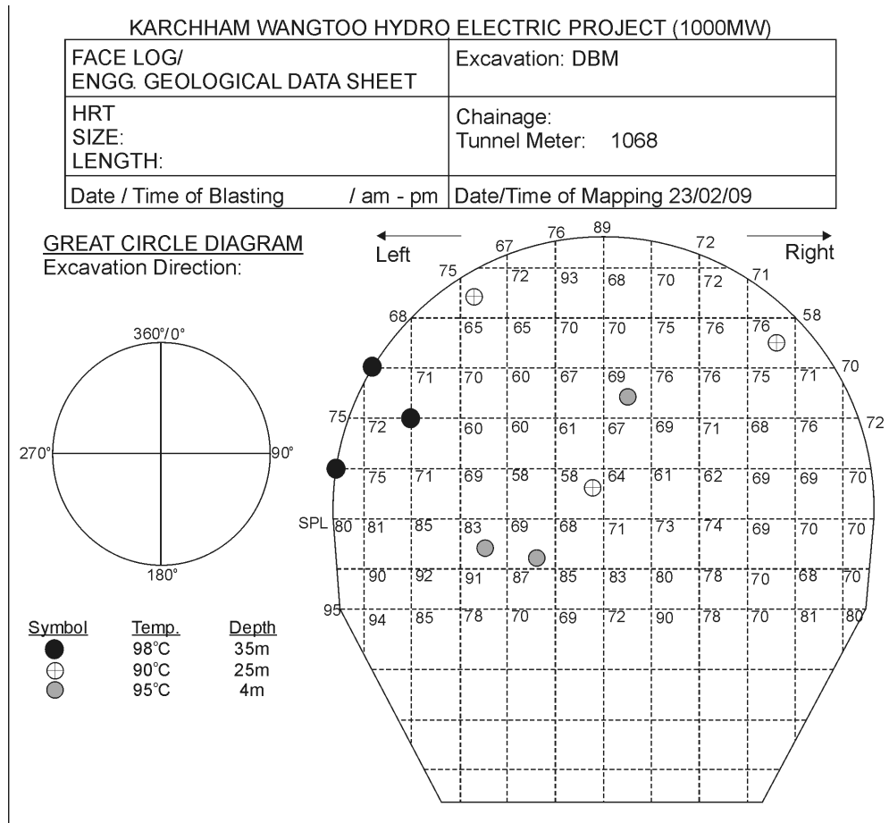
Fig.3 - Temperature log in degree celcius of the face, Adit-4 (Upstream), KWHEP, H.P.
