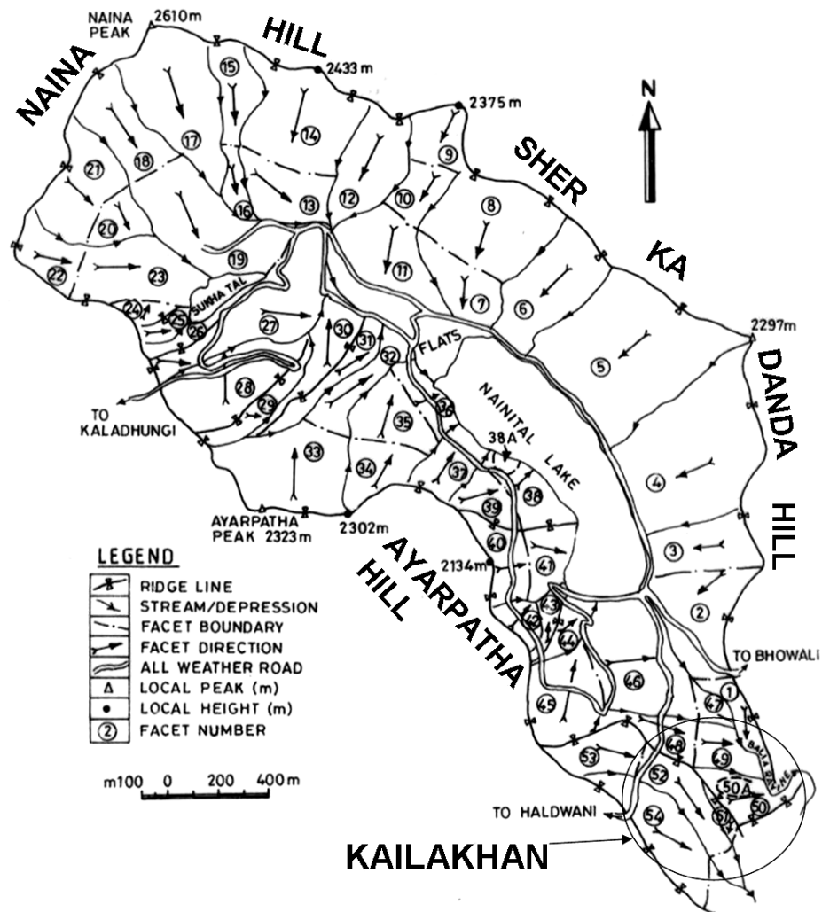
Fig. 3 - Slope facet map of study area Nainital
