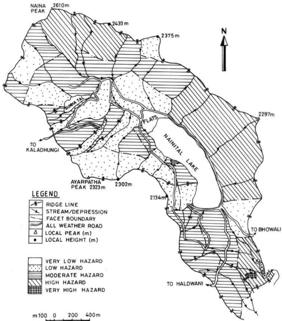
Fig. 4 - Landslide hazard zonation (LHZ) map of the Nainital area
