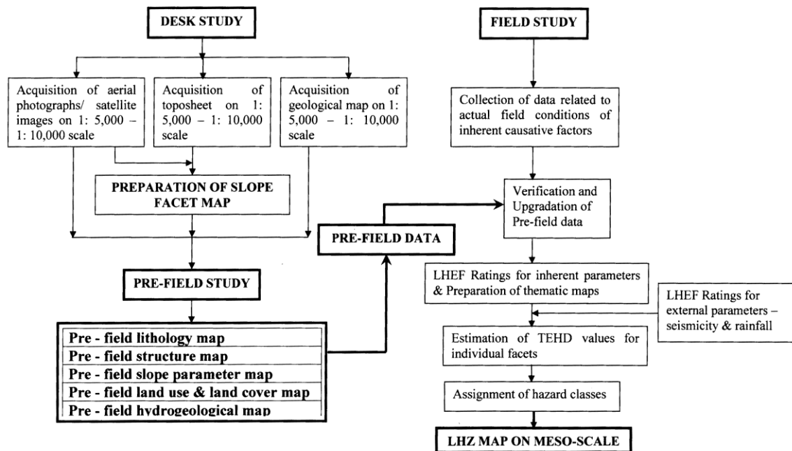
Fig. 1 - Flow chart showing methodology of meso-scale LHZ mapping technique
