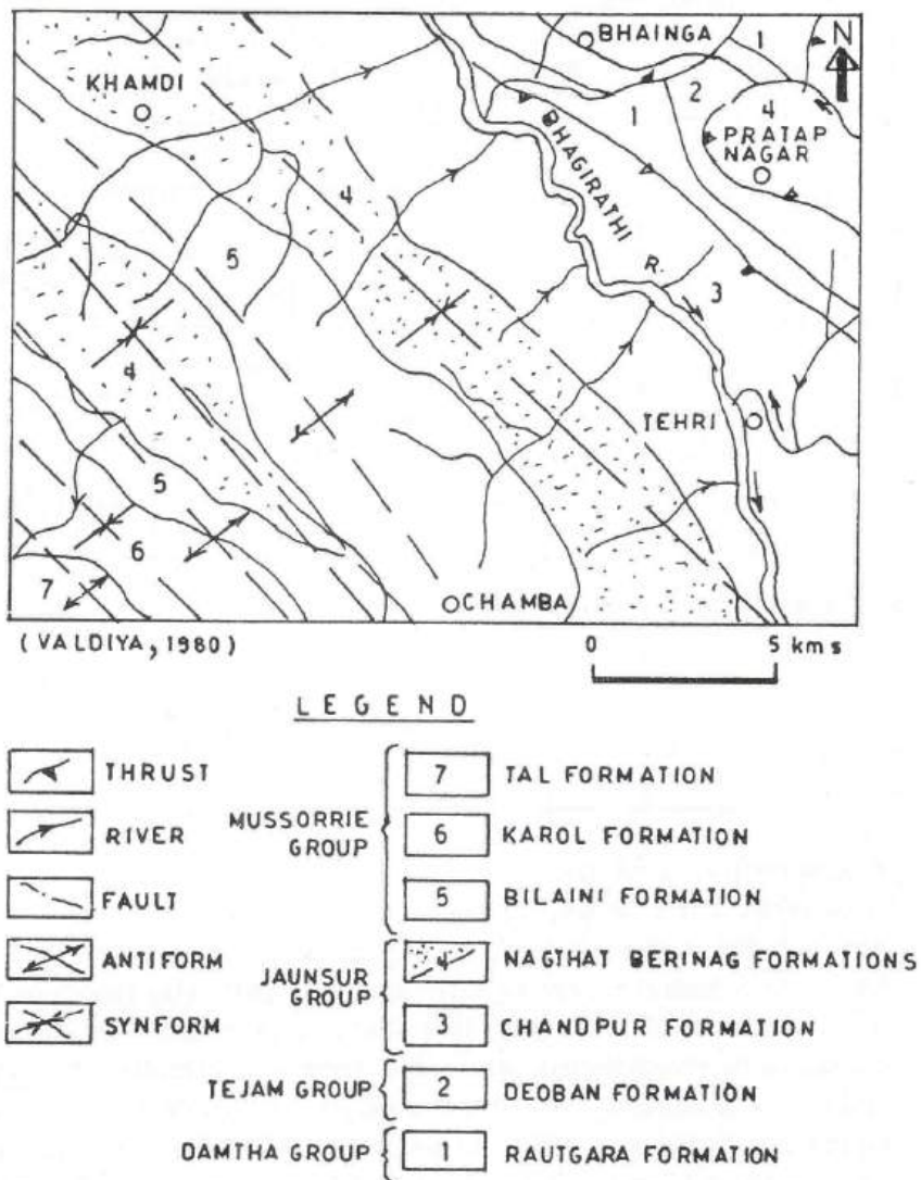
Fig. 2. Geological map of the study area
